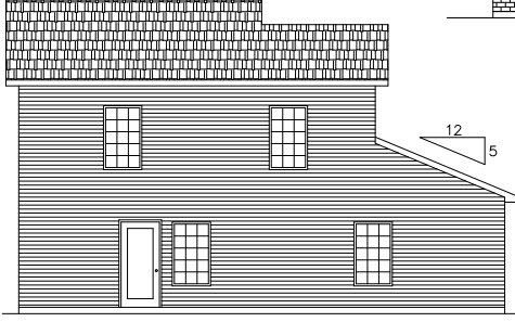
BACK ELEVATION SCALE = 1/8"=1'-0"
